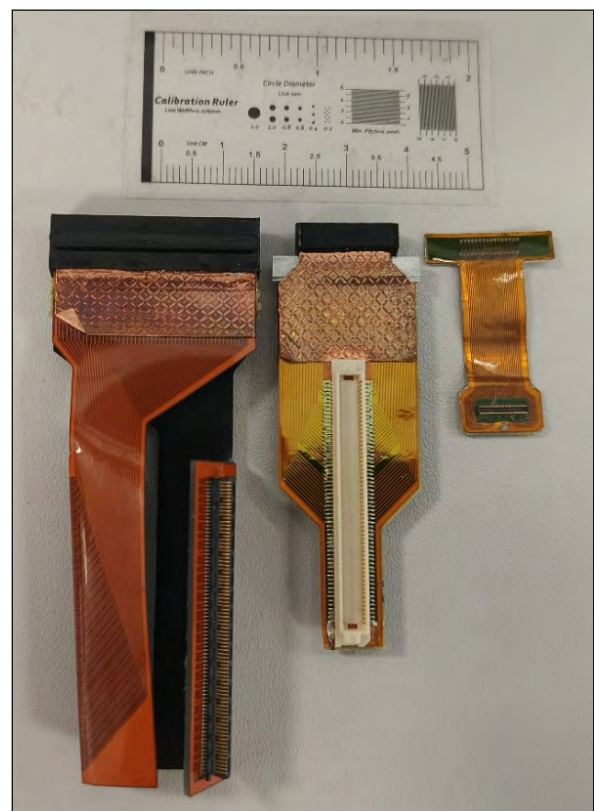
Fig. 1. Evaluated arrays (left to right): 14 MHz rigid, 28 MHz single-crystal, and 25 MHz flexible with integrated PCB. Ruler for scale.
