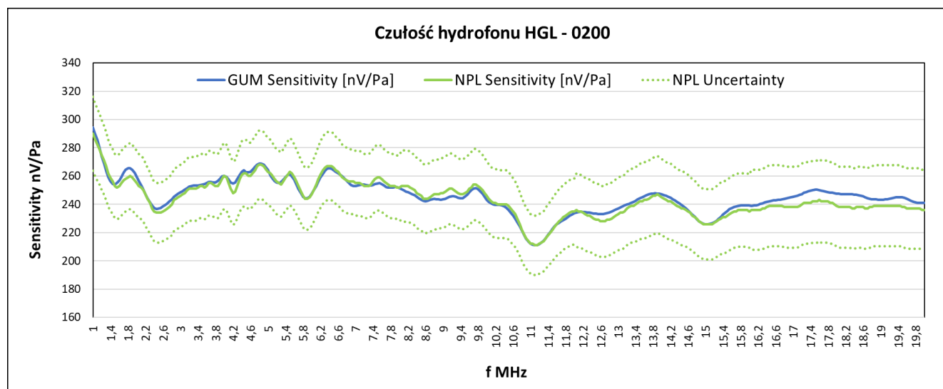
Fig. 1. The sensitivity of the HGL-0200 hydrophone.
