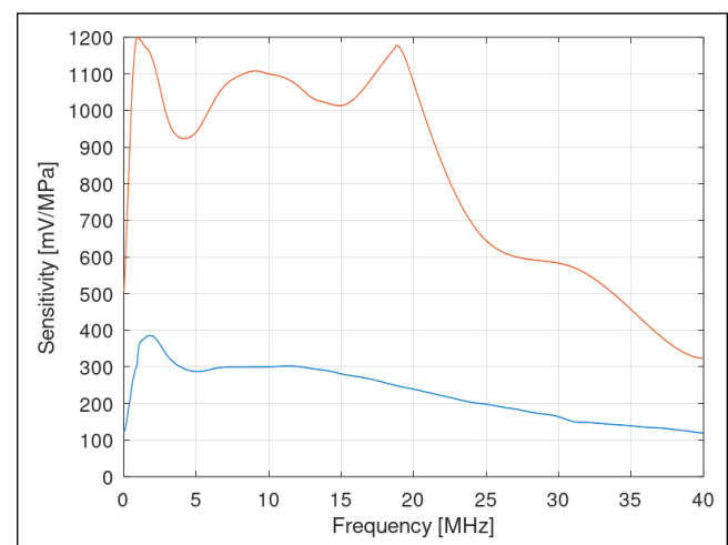
Fig. 1. Frequency Spectra of the Hydrophones; Red: CMUT-Hydrophone 0.5 x 0.5 mm 2 , 250Pa NEP; Blue: Commercially available Piezo-Hydrophone \varnothing 0.5 mm, 200Pa NEP (NH0500 from Precision Acoustics Ltd.).
