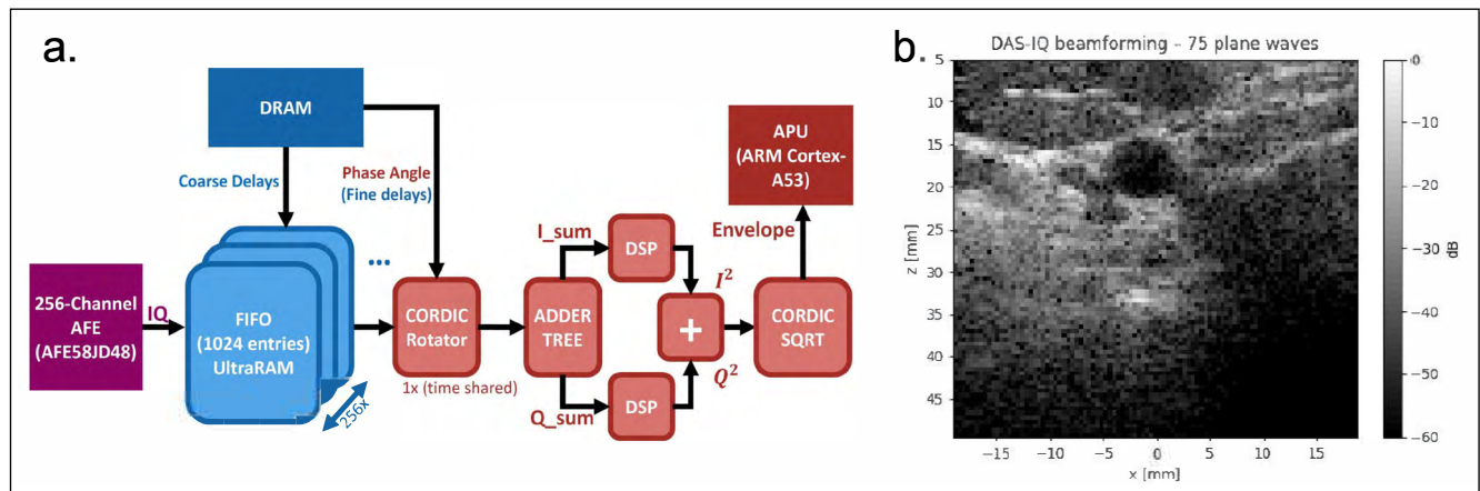
a. Soc reconstruction chain overview.
