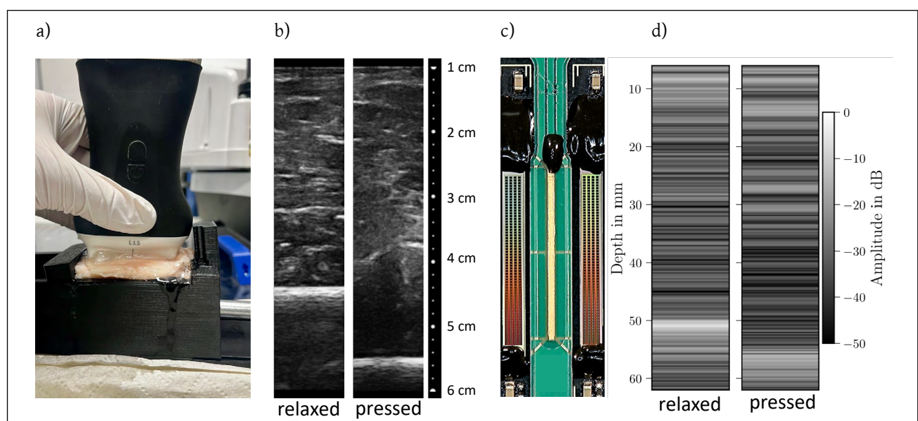
a) Muscle press with Clarius; b) B-Mode (Clarius); c) Hybrid Stack; d) A-Scan from Hybrid Stack
