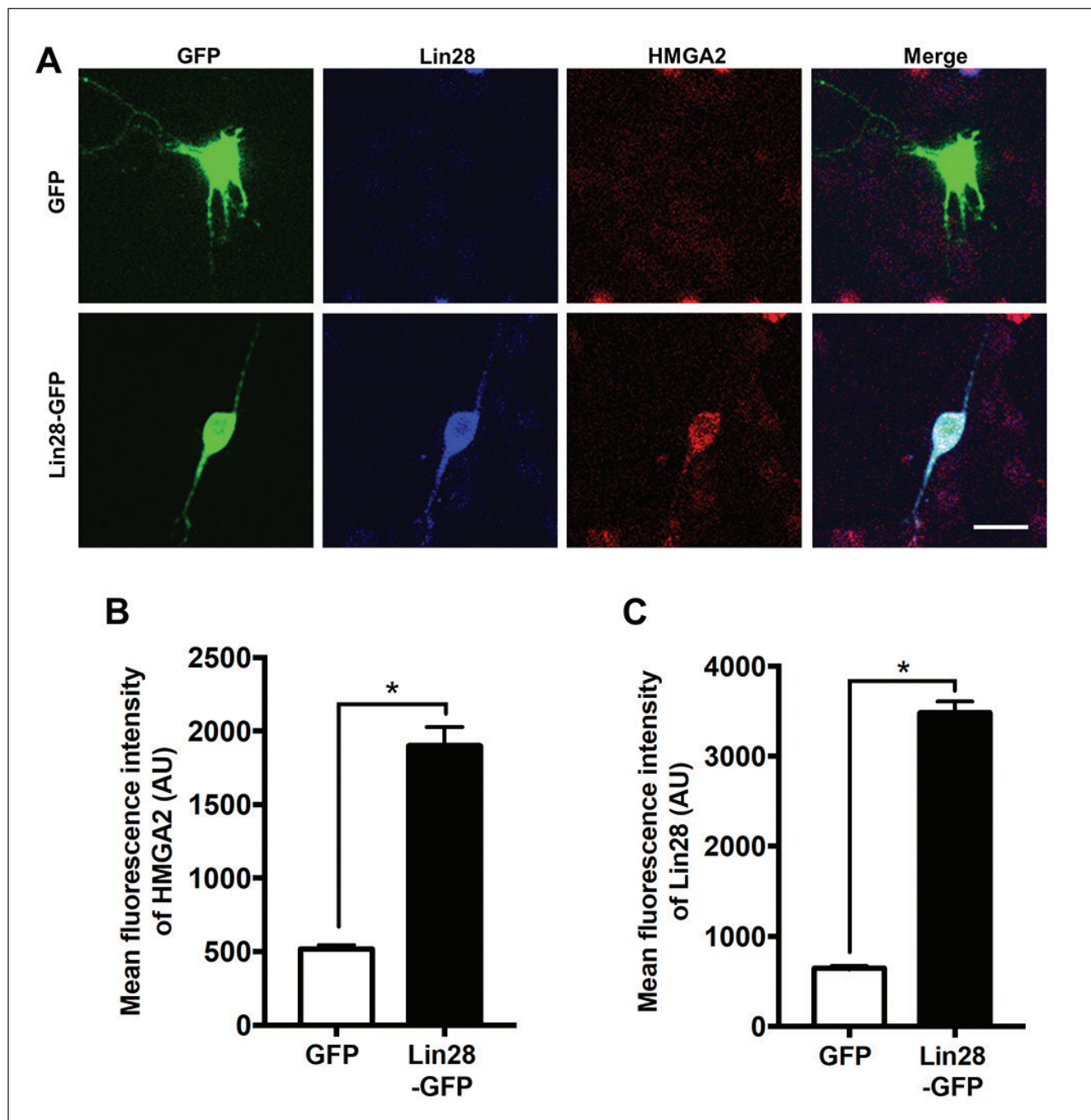
Fig. 3. Lin28-GFP overexpression induced high mobility group AT-hook 2 (HMGA2) expression. (A) Representative fluorescent images showing GFP (green), Lin28 (blue), and HMGA2 (red) expression in electroporated cells. Scale bar=20 \mu m. (B) A graph showing mean fluorescence intensity of HMGA2 immunoreactivity. Note that HMGA2 expression was significantly increased in Lin28-GFP-overexpressing cells. * p < 0.05 by Mann-Whitney U test between GFP- and Lin28-GFP-electroporated cells. Sample size for each group is 25. Data represent mean \pm S.E.M. (C) A graph showing mean fluorescence intensity of Lin28 immunoreactivity. Note that Lin28 expression was significantly increased in Lin28-GFP-overexpressing cells, whereas no signal was detected in GFP-expressing controls. * p < 0.05 by Mann-Whitney U test between GFP- and Lin28-GFP-electroporated cells. Sample size for each group is 25. Data represent mean \pm S.E.M.
