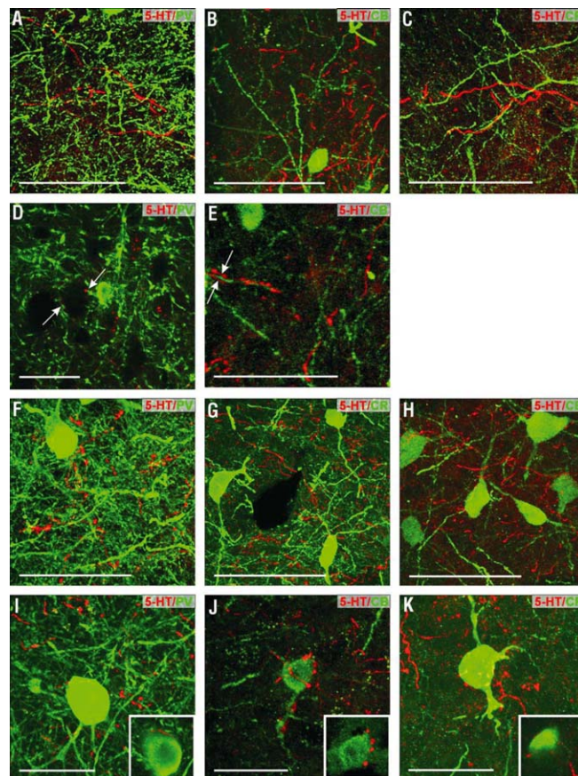
Fig. 4. Photomicrographs of the immunoreactivity for calcium binding proteins and 5-HT. Left column – parvalbumin, middle column – calbindin, right column – calretinin. There was no colocalization of 5-HT with the calcium binding proteins within fibers (A–C). 5-HT- and PV-ir terminals on the surface of the non-labeled cell (basket, D, arrows). 5-HT-ir terminals on CB-ir fibers (arrows, E). 5-HT fibers in the close vicinity of cell bodies containing the studied calcium binding proteins (F–H). Direct contacts of the 5-HT-immunoreactive fibers (I) and terminals (J–K) with cells containing CaBPs. Stacks of confocal images. Lower-left corner photomicrograph shows one 0.05 \mu\text{m} layer. Scale bar equals to 50 \mu\text{m} (A–H) and 25 \mu\text{m} (I, K).
